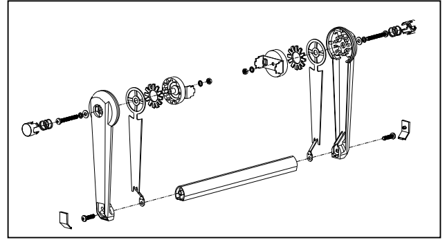
Explode view for T1 or T2
