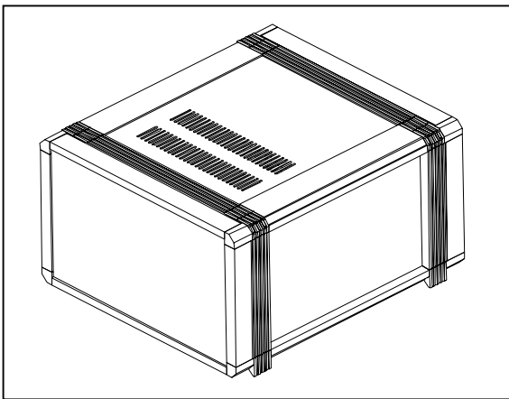
Cut-outs or special vent holes in the top and bottom cover
